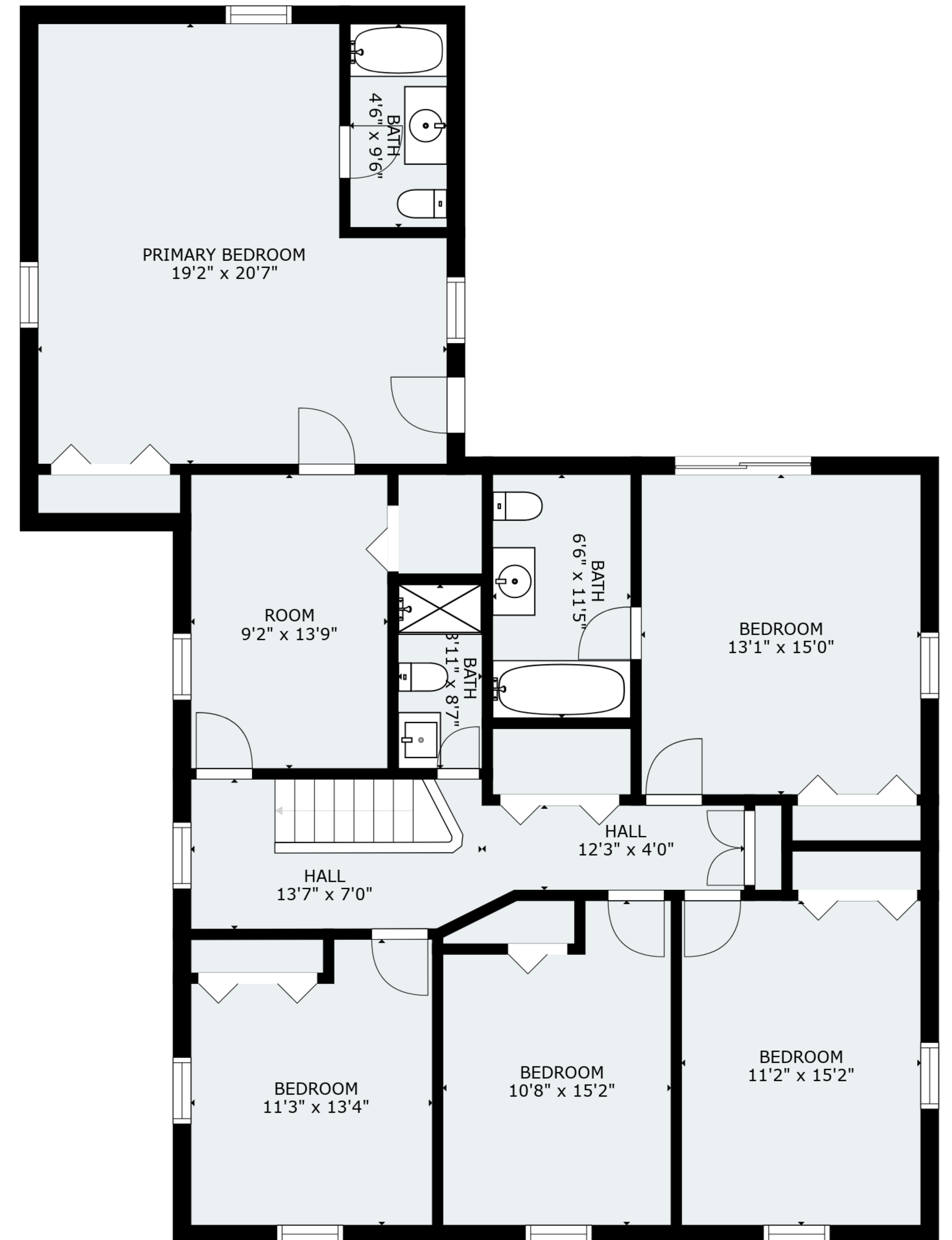
FLOOR 2
