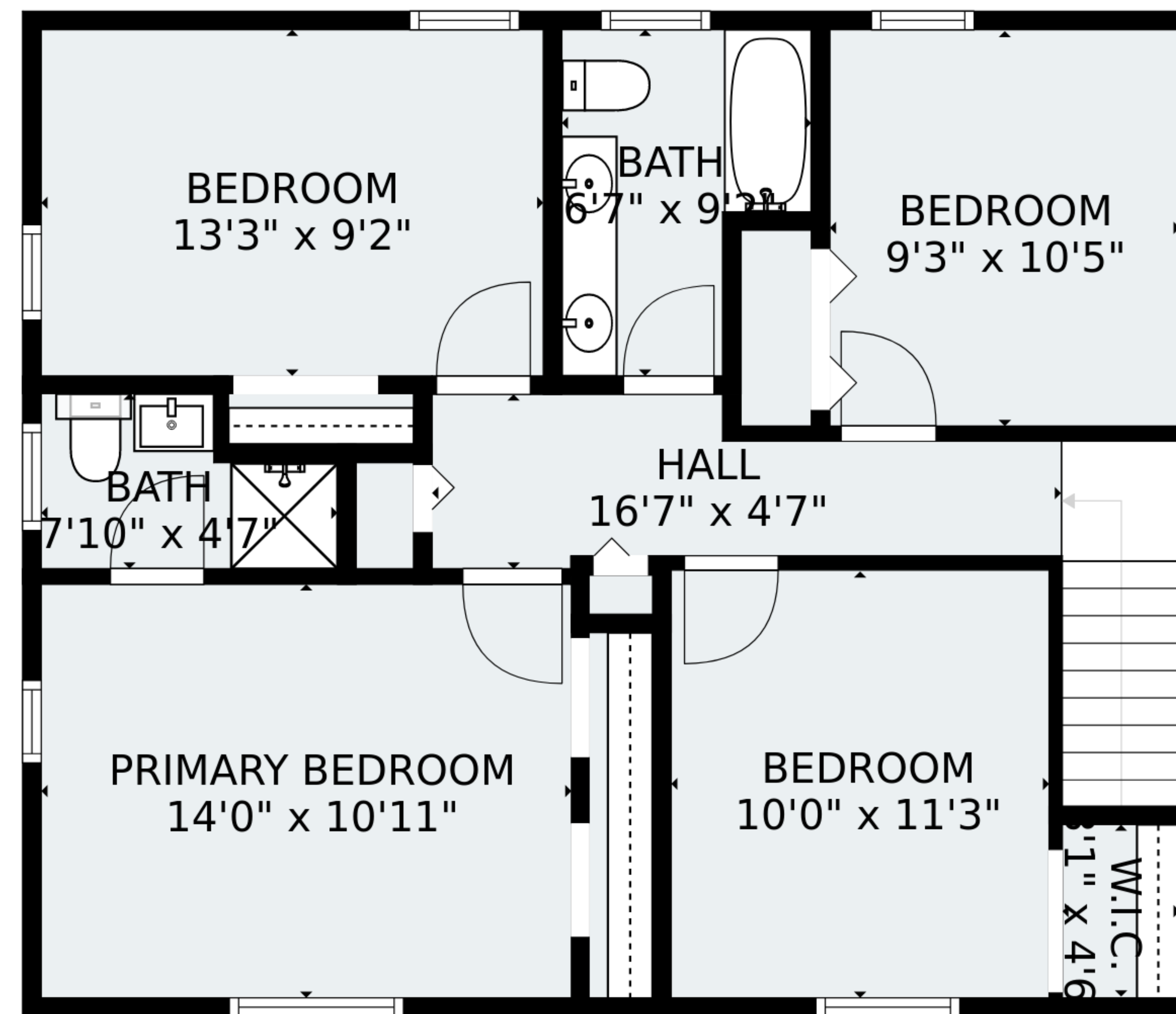
FLOOR 3
