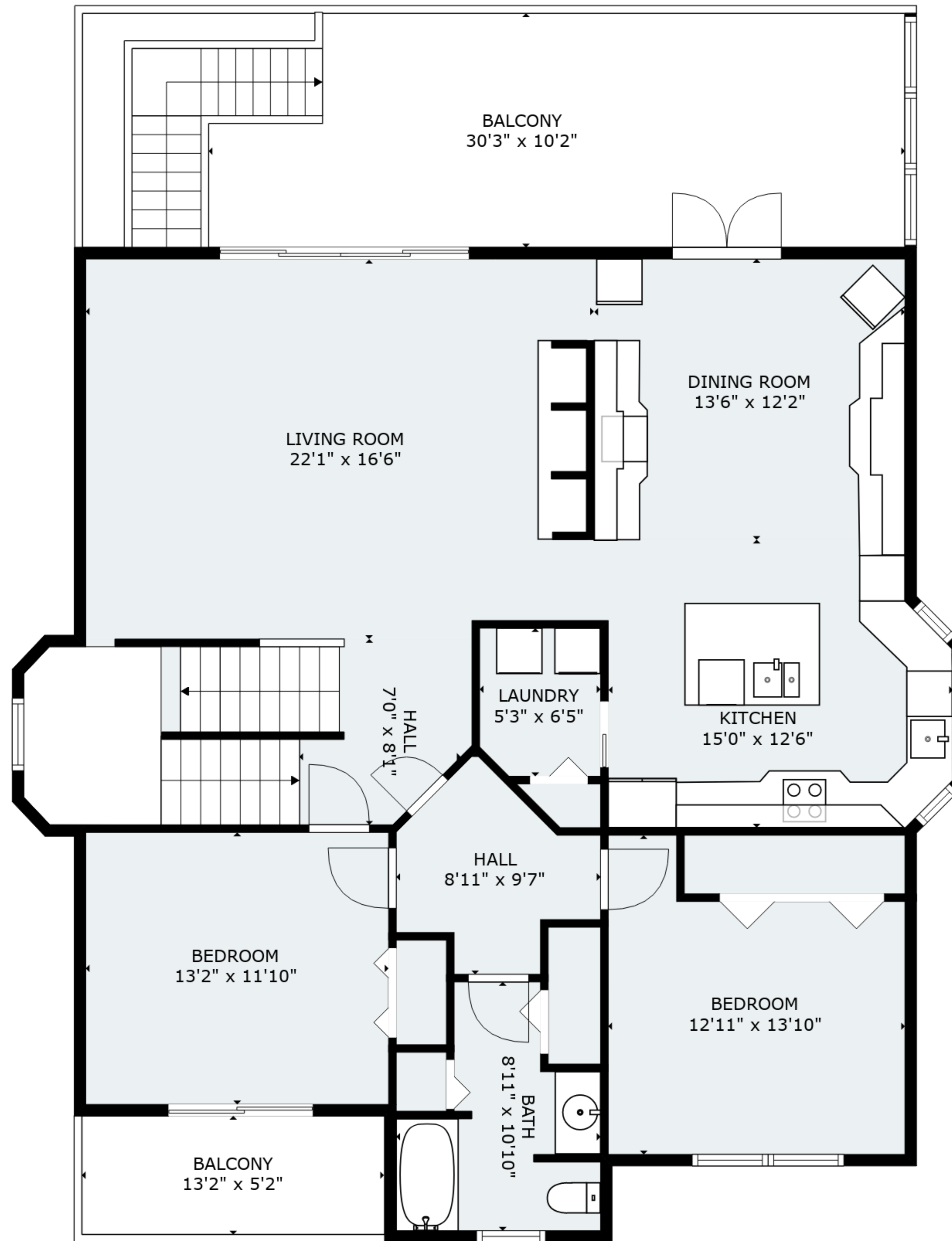
FLOOR 2
