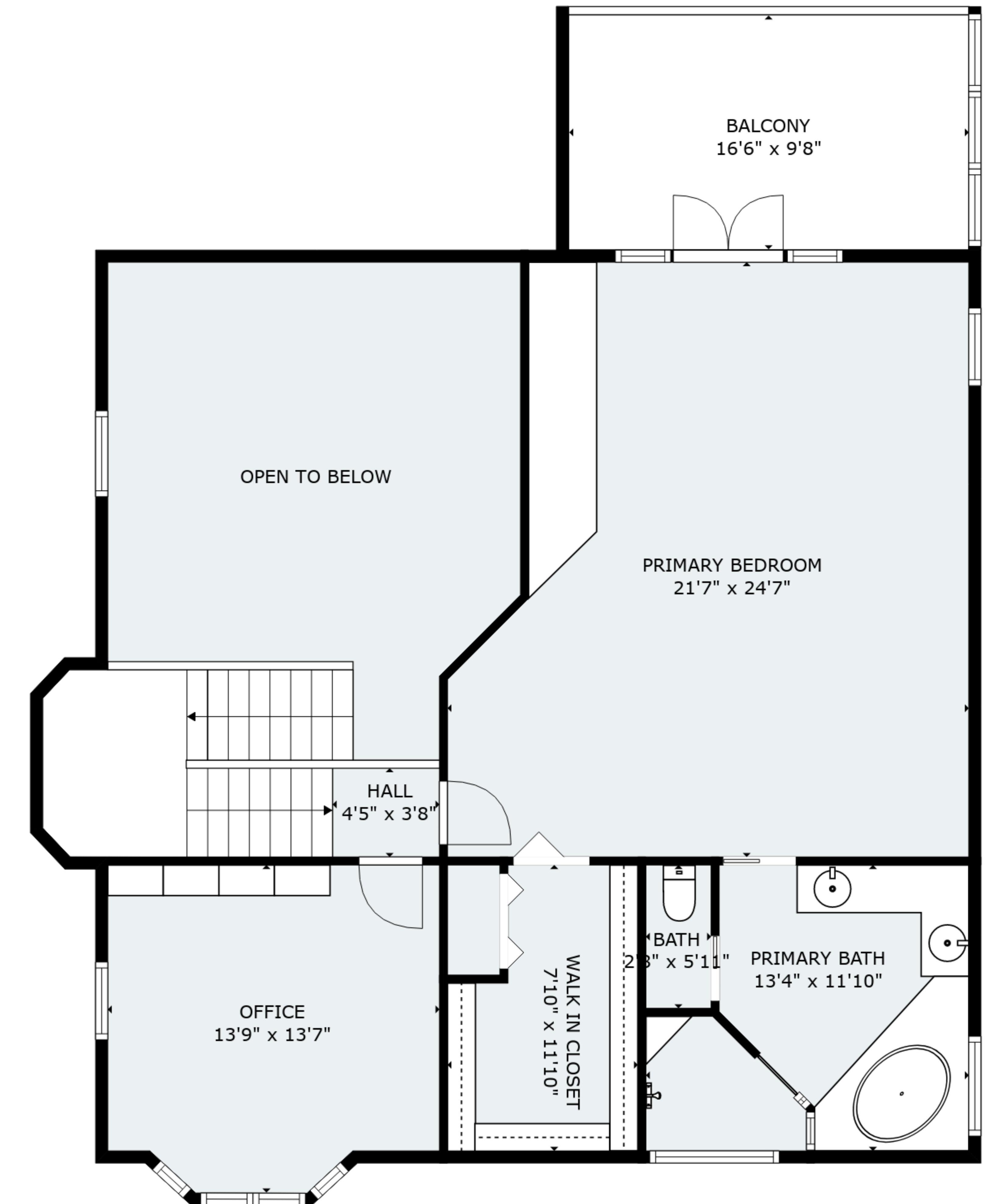
FLOOR 3
