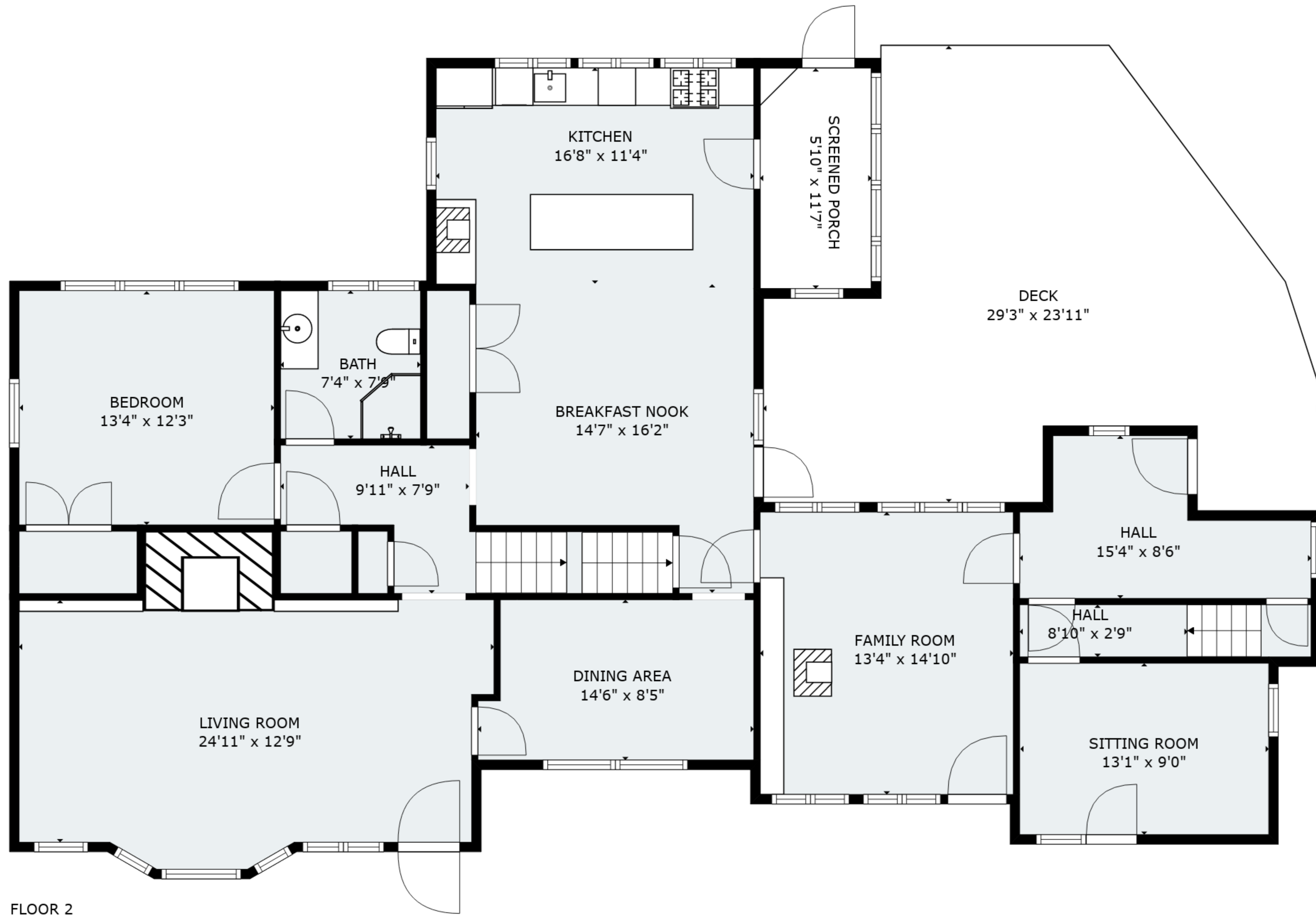
FLOOR 2
