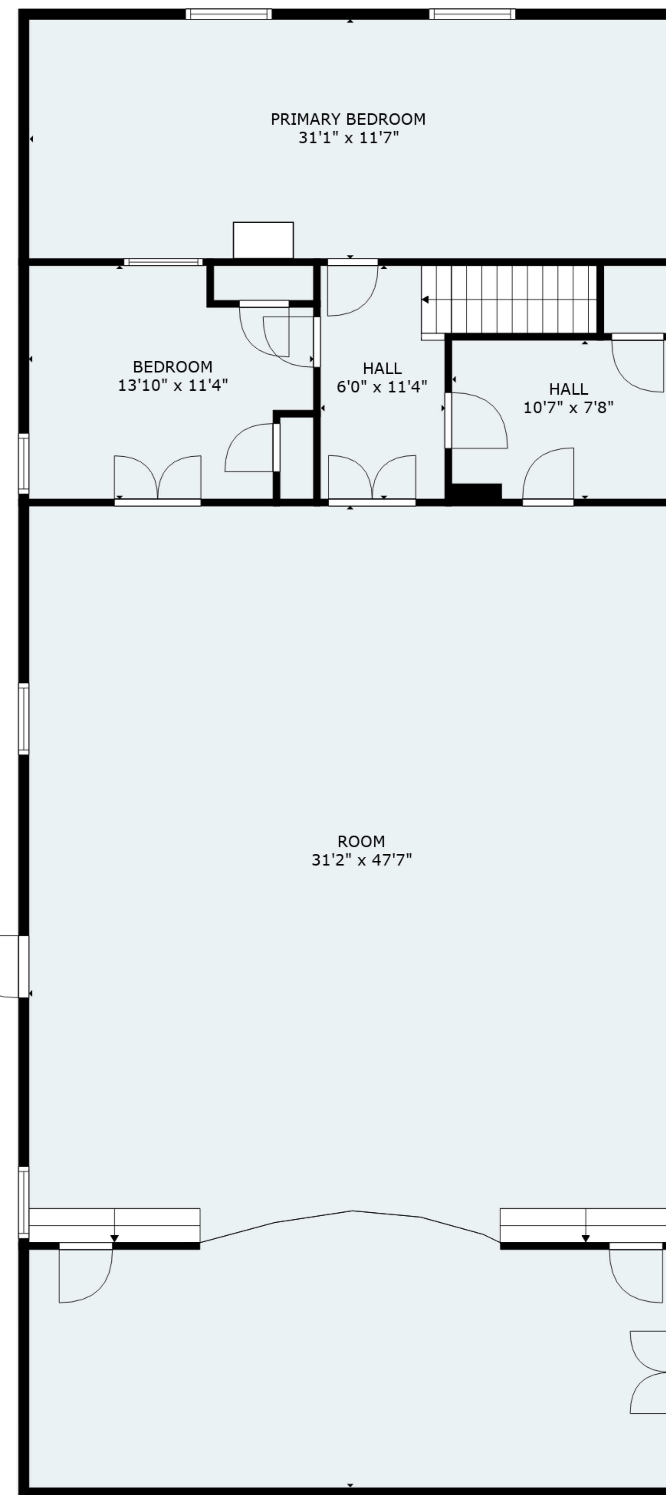
FLOOR 3
