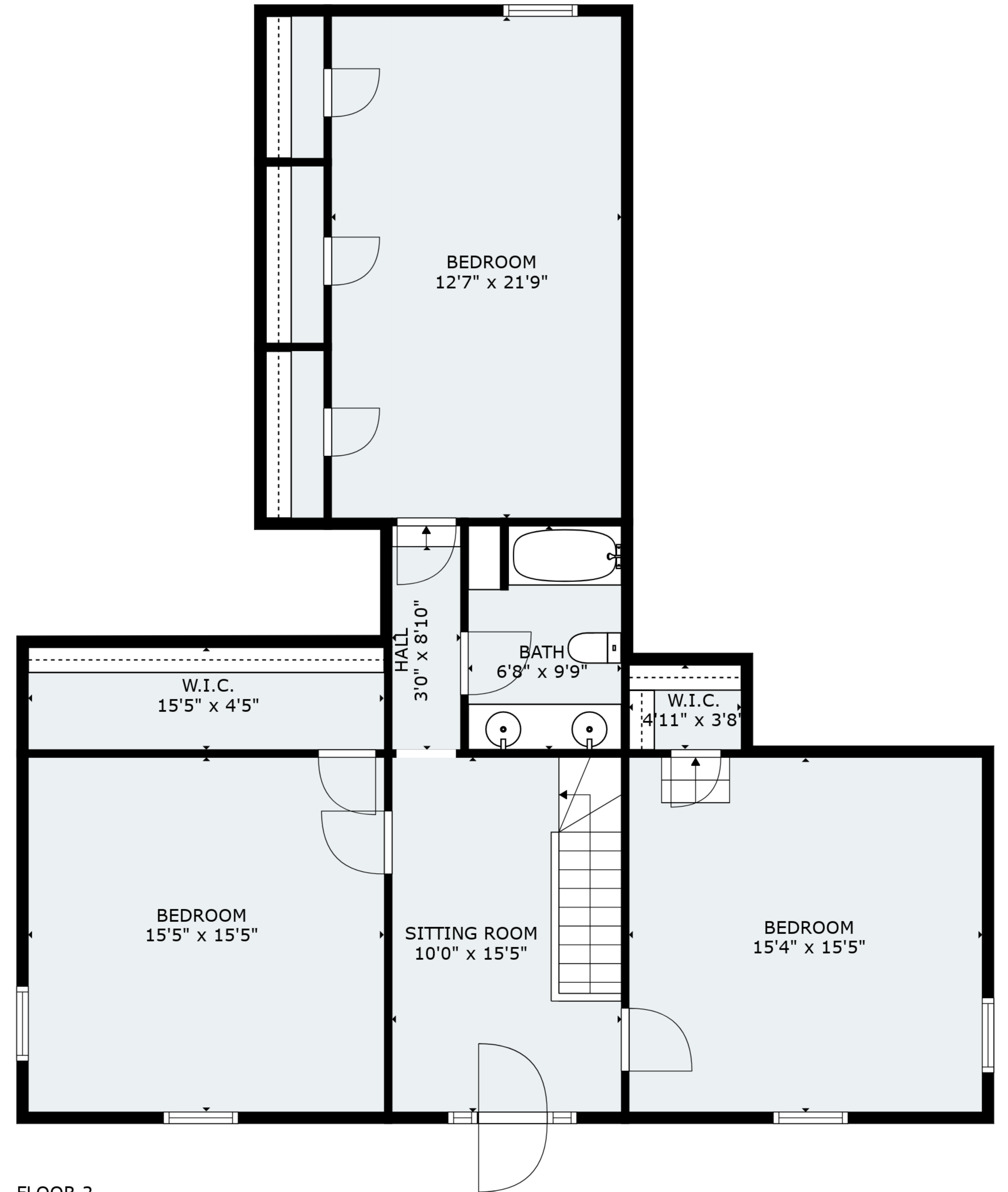
FLOOR 2
