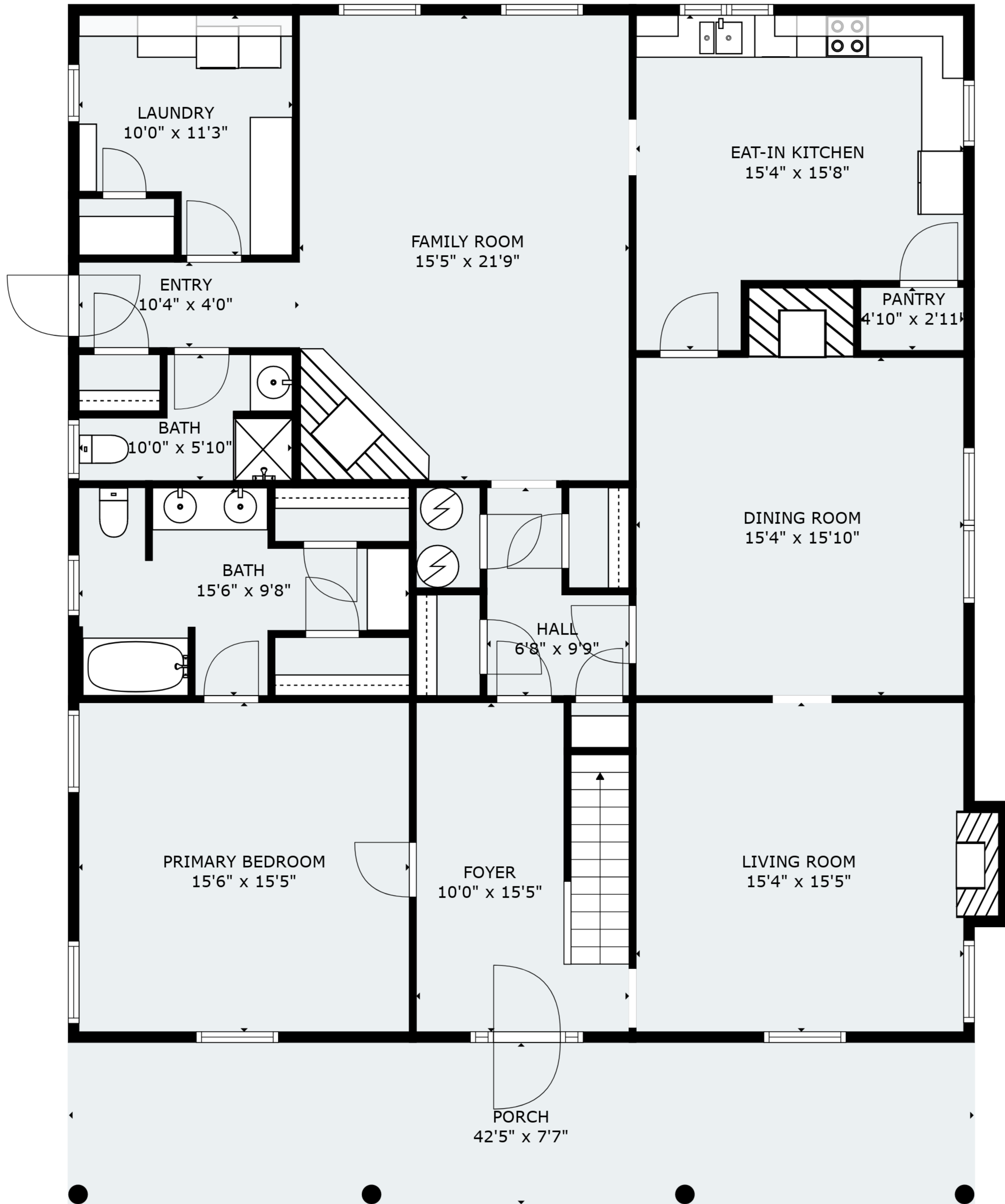
FLOOR 1
