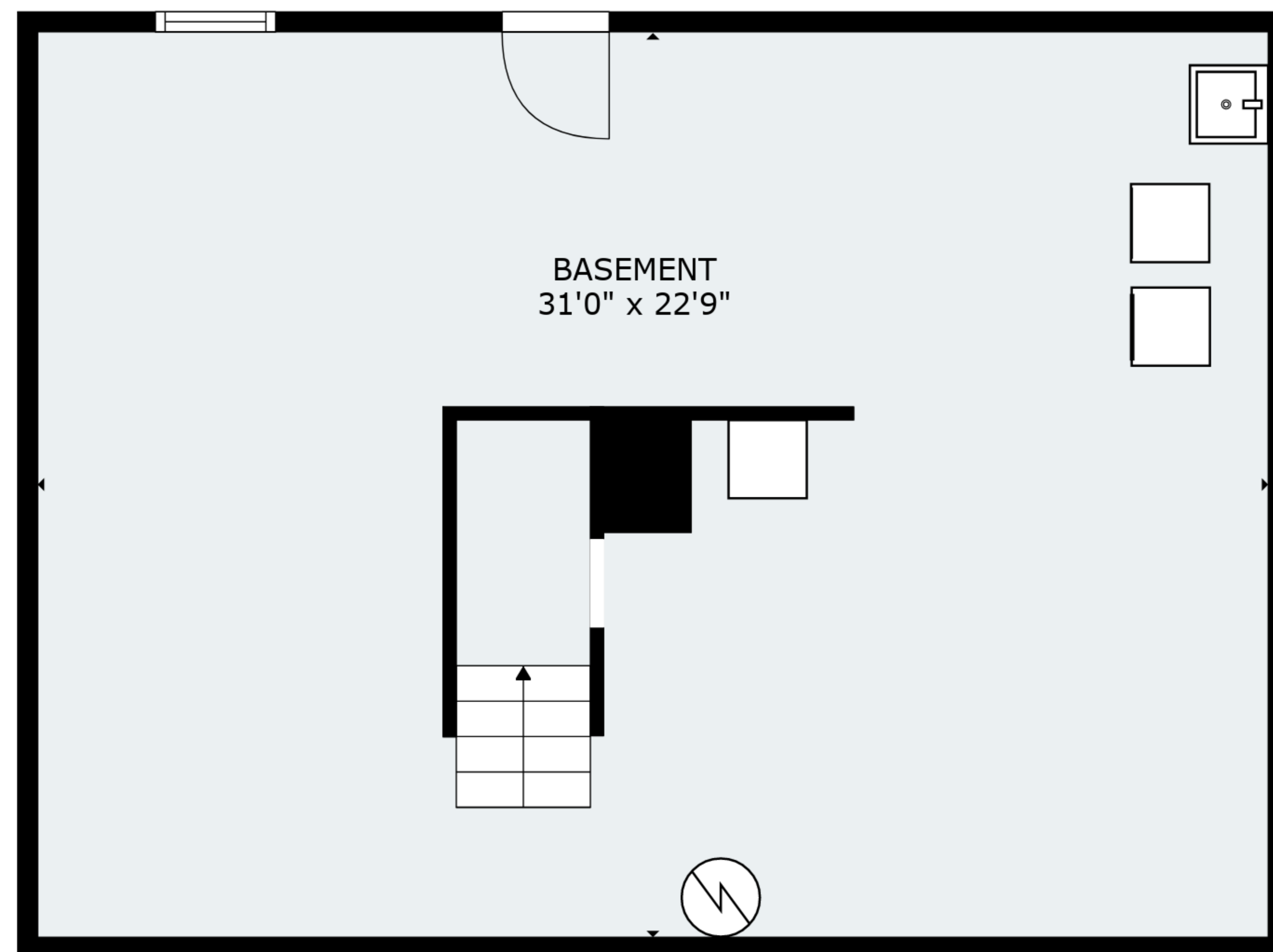
FLOOR 1
