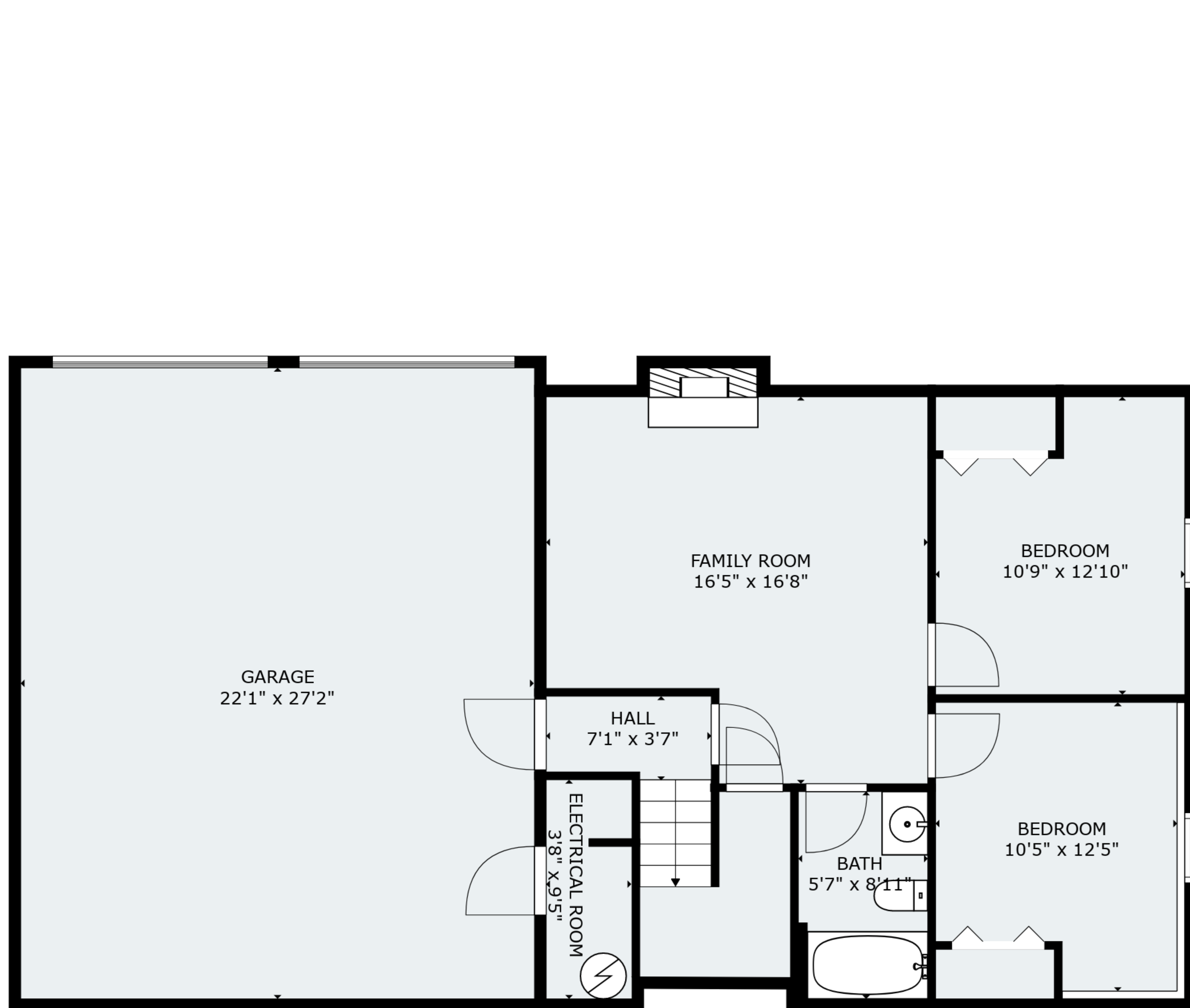
FLOOR 1
