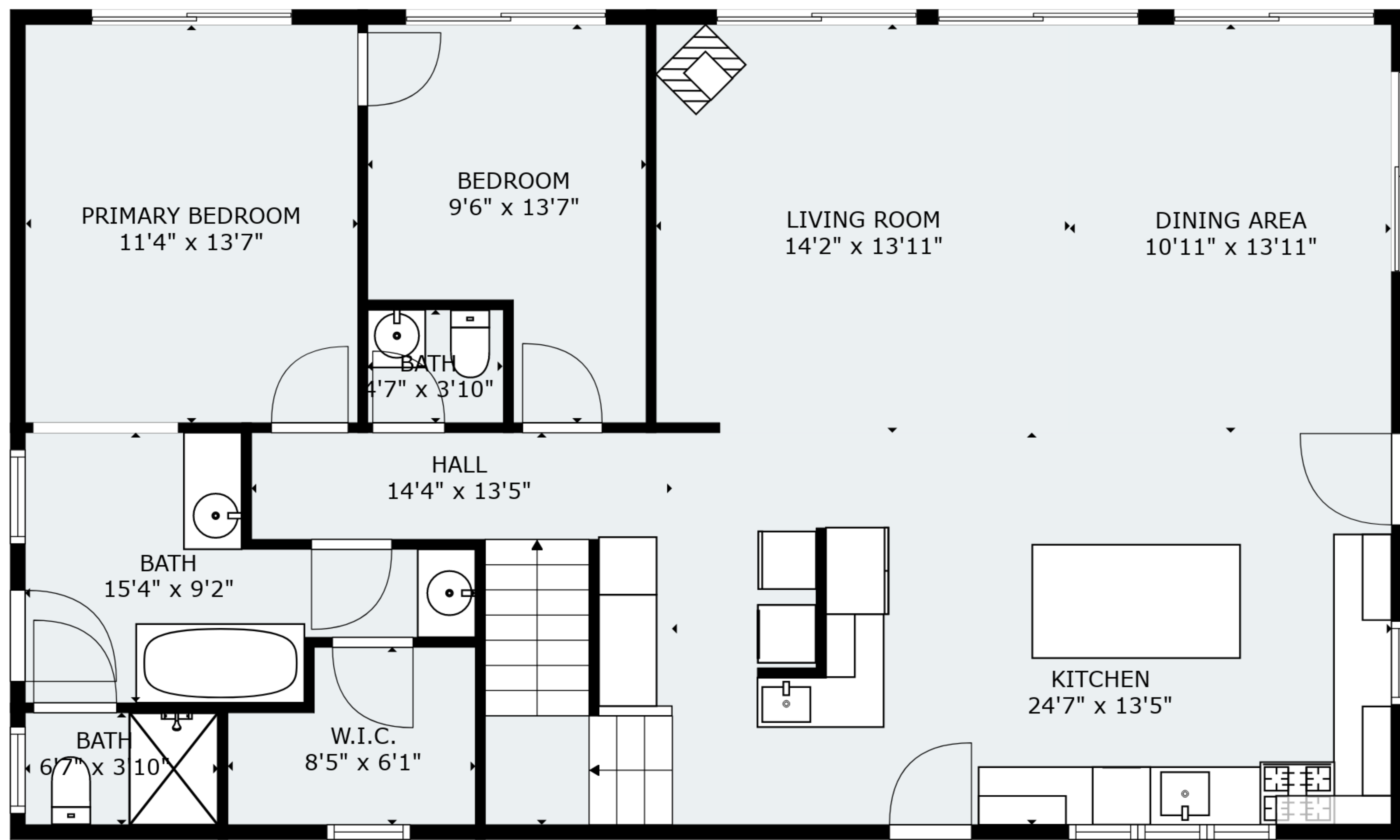
FLOOR 2
