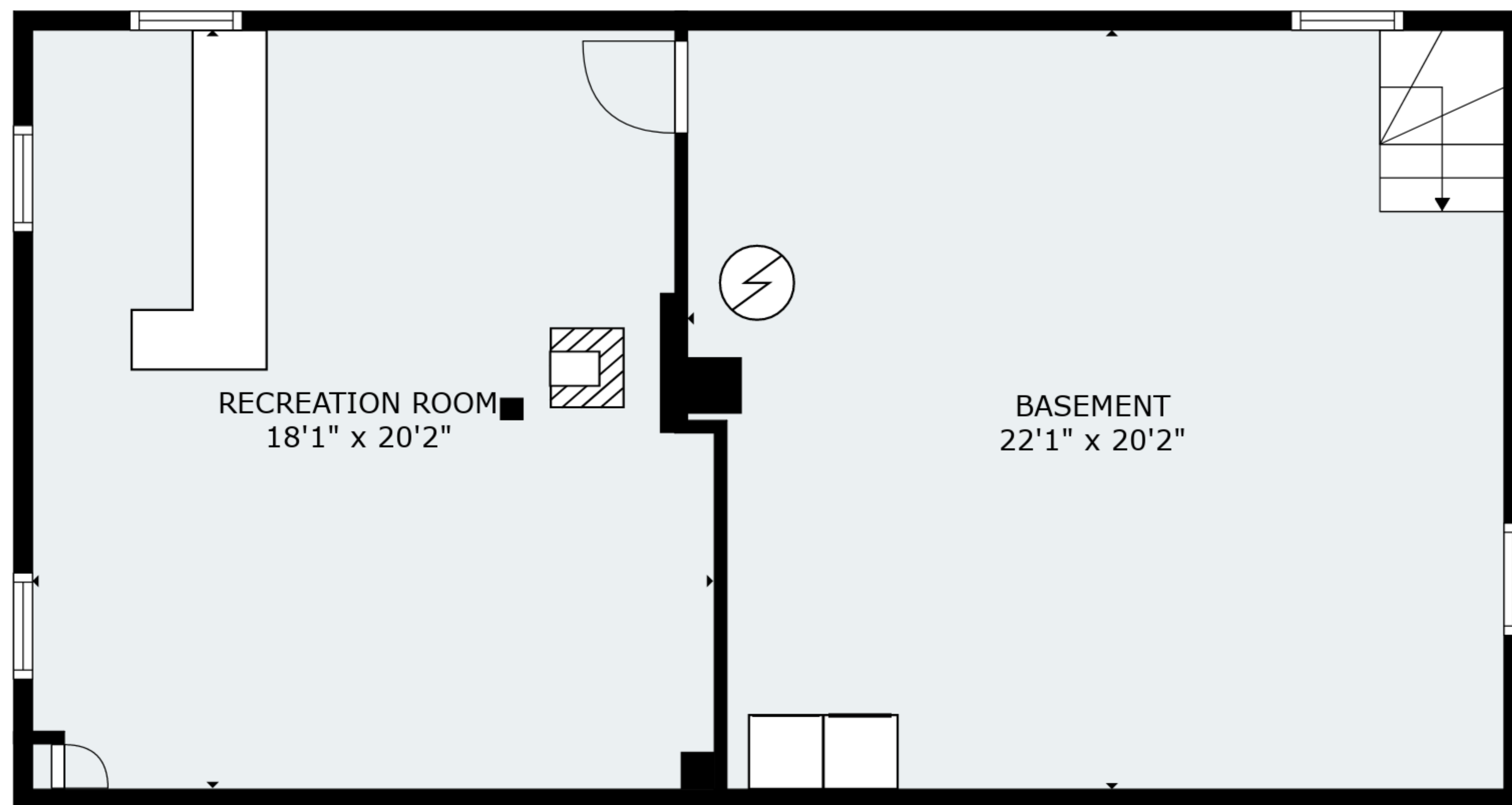
FLOOR 1
