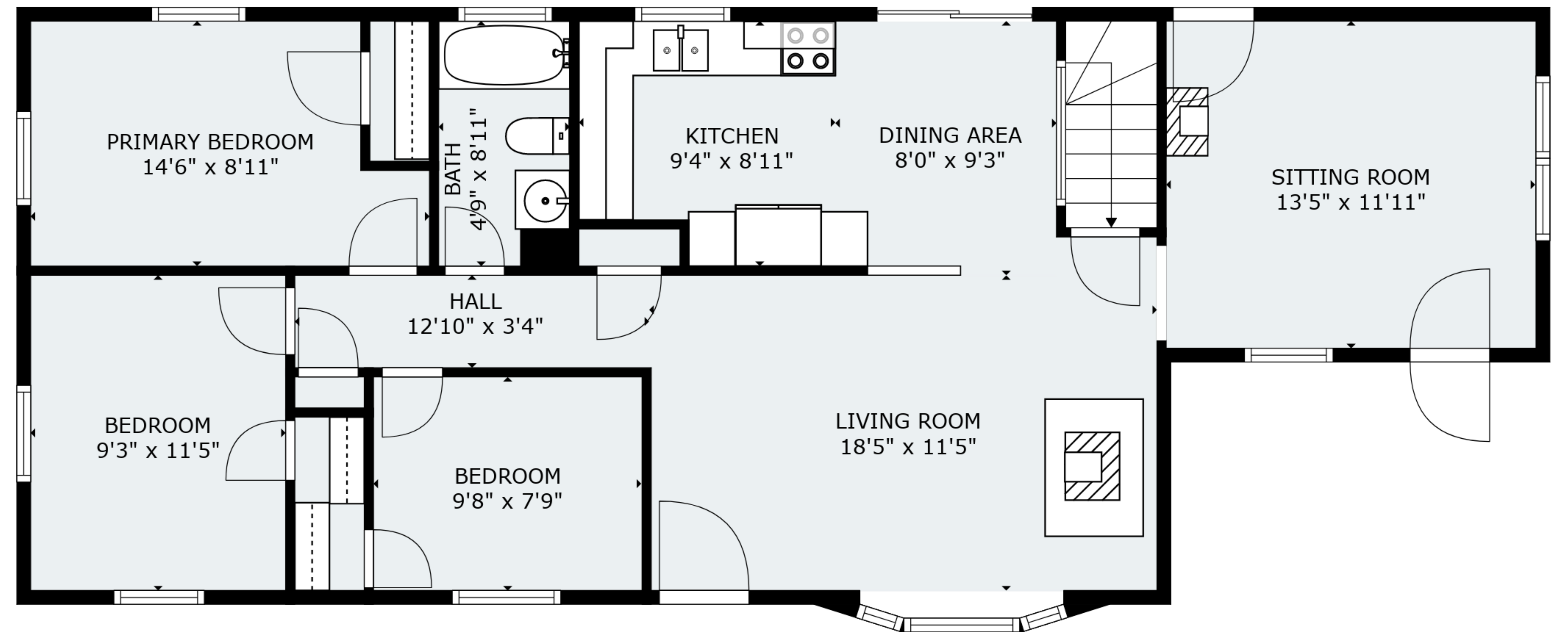
FLOOR 2
