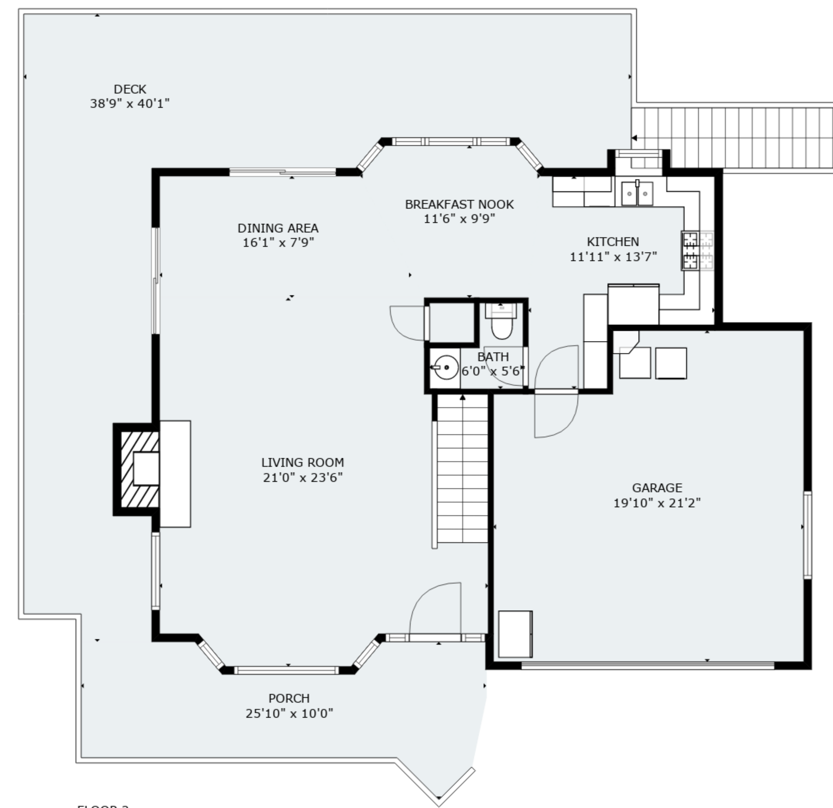
FLOOR 2
